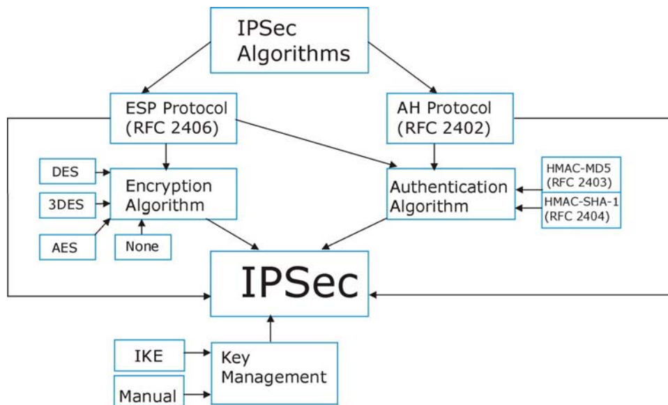
Figure 138 IPSec Architecture
