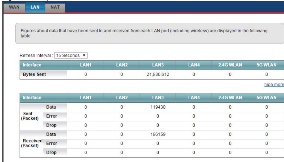
Figure 160 System Monitor > Traffic Status > LAN
