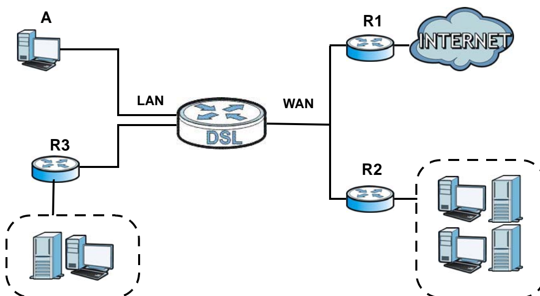
Figure 62 Example of Routing Topology
