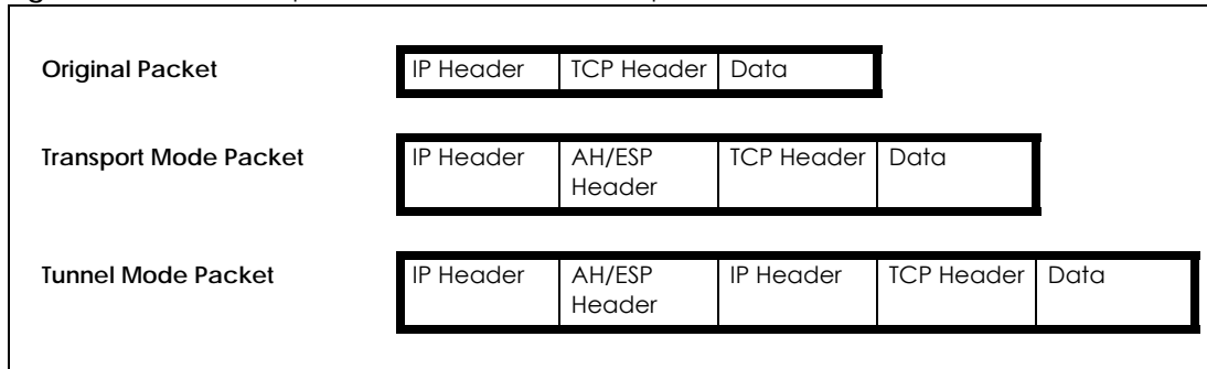
Figure 254 VPN: Transport and Tunnel Mode Encapsulation
