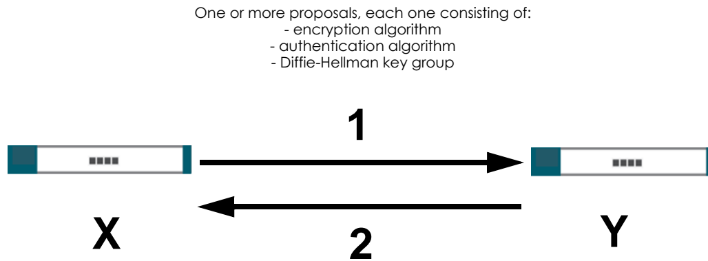
Figure 250 IKE SA: Main Negotiation Mode, Steps 1 - 2: IKE SA Proposal
