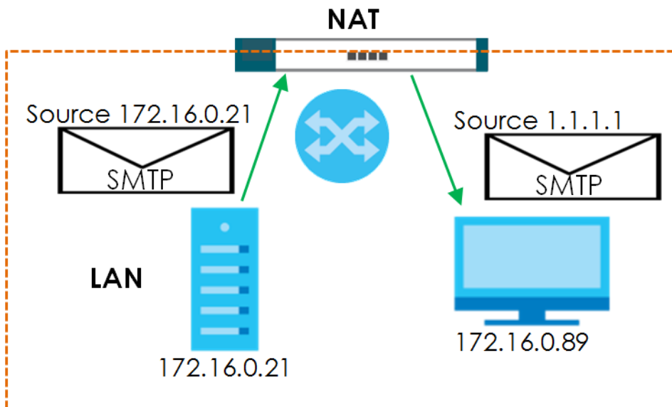
Figure 151 LAN to LAN Return Traffic
