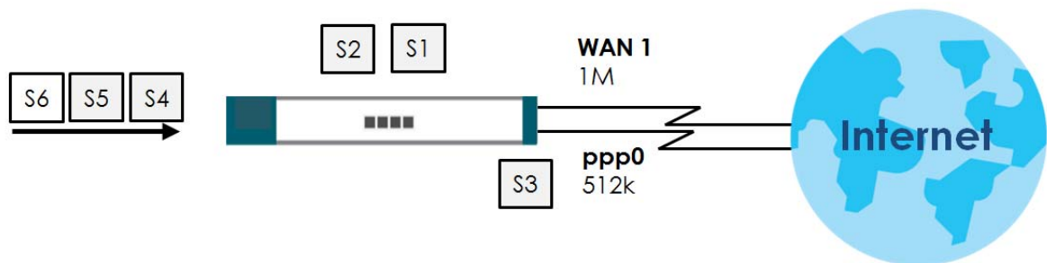
Figure 134 Weighted Round Robin Algorithm Example
