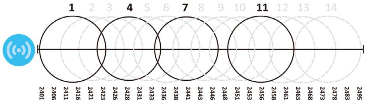
Figure 112 An Example Four-Channel Deployment
