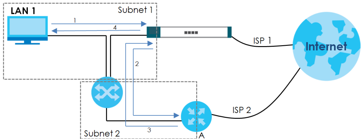
Figure 211 Using Virtual Interfaces to Avoid Asymmetrical Routes
