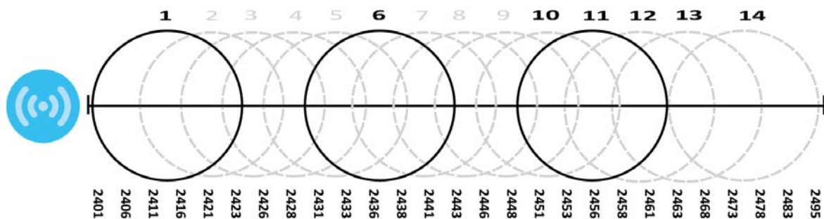
Figure 111 An Example Three-Channel Deployment
