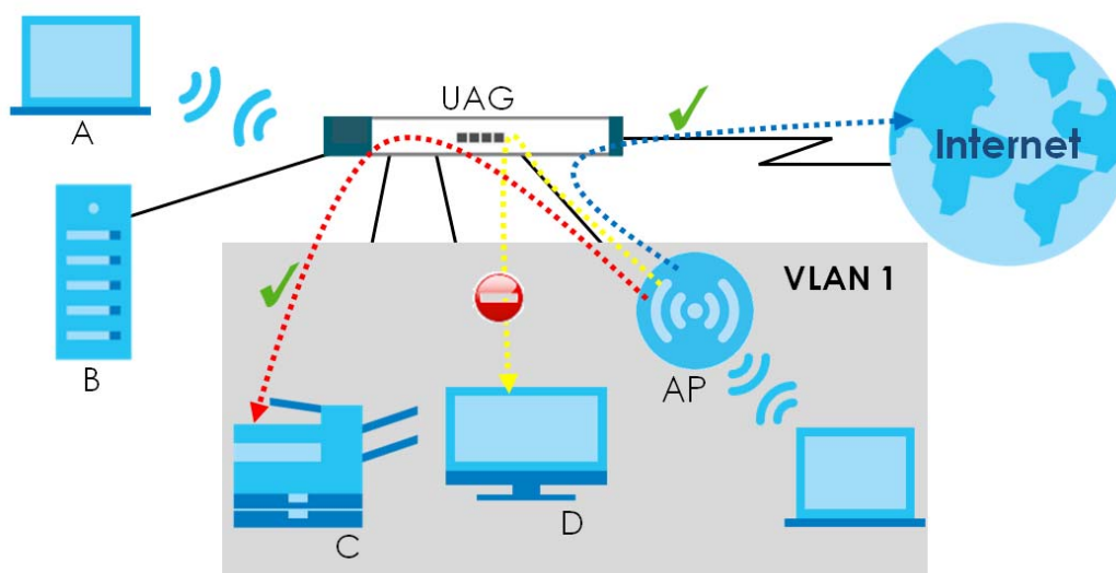
Figure 178 Layer-2 Isolation Application
