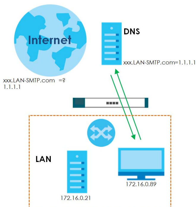
Figure 149 LAN Computer Queries a Public DNS Server
