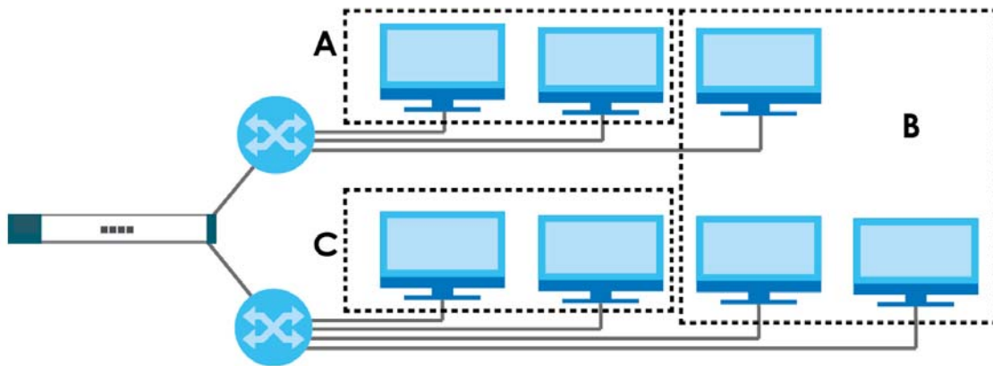
Figure 125 Example: Before VLAN
