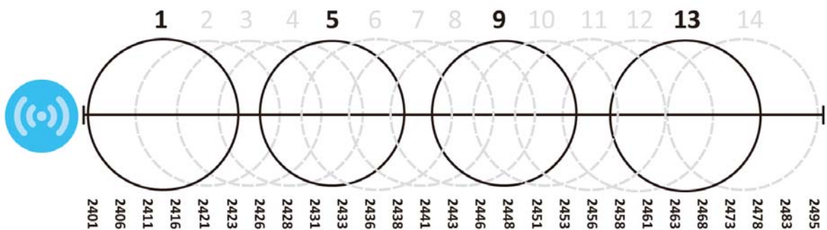
Figure 113 An Alternative Four-Channel Deployment
