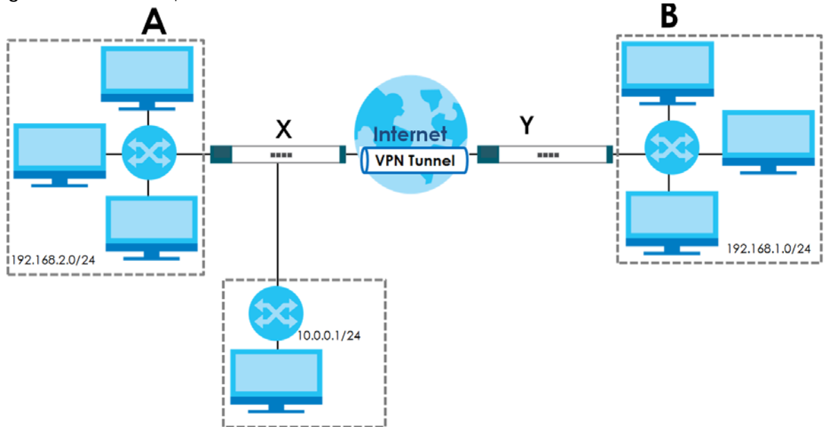
Figure 255 VPN Example: NAT for Inbound and Outbound Traffic
