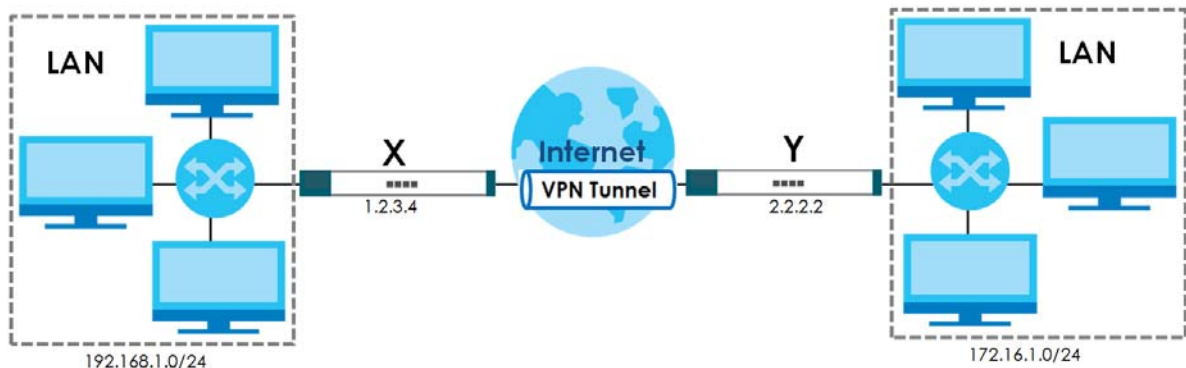
Figure 256 IPsec VPN Example
