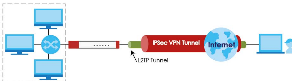
Figure 30 L2TP VPN Overview
