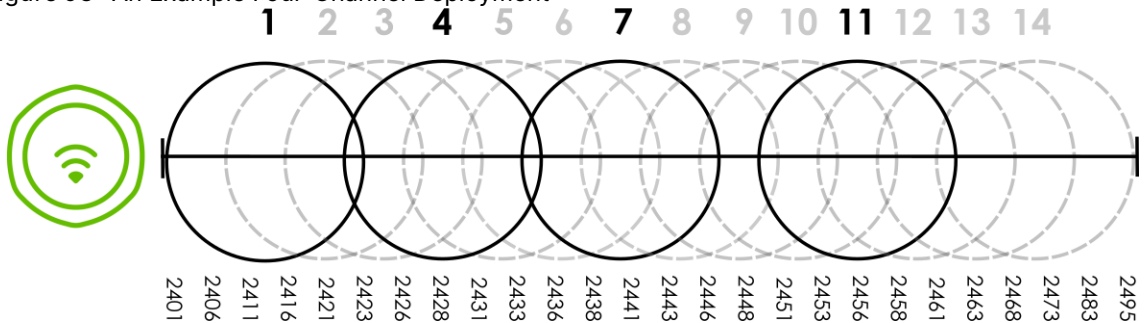
Figure 93 An Example Four-Channel Deployment
