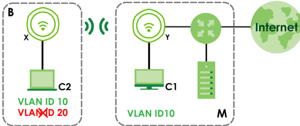
Figure 79 Wireless Bridge VLAN ID Example
