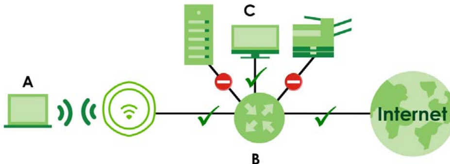
Figure 121 Layer-2 Isolation Application
