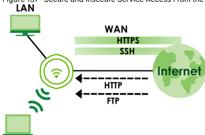
Figure 137 Secure and Insecure Service Access From the WAN
