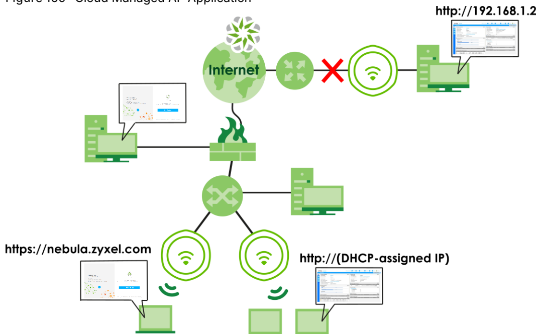
Figure 169 Cloud Managed AP Application
