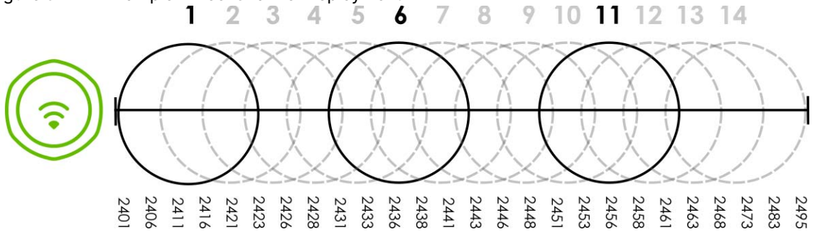
Figure 92 An Example Three-Channel Deployment
