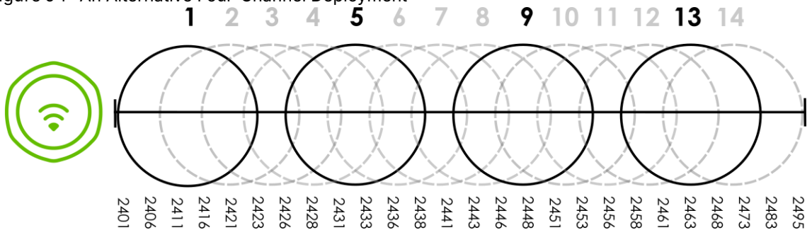
Figure 94 An Alternative Four-Channel Deployment
