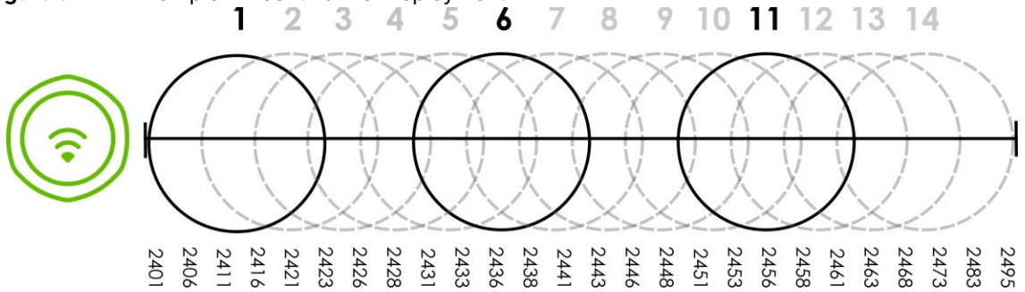
Figure 94 An Example Three-Channel Deployment
