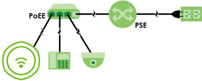
Figure 36 PoE Example Application - PSE with PoE Extender
