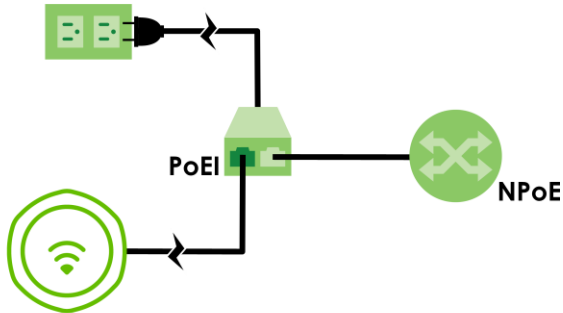
Figure 37 PoE Example Application - PoE Injector
