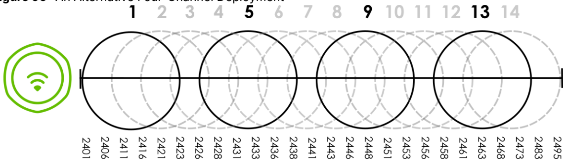
Figure 96 An Alternative Four-Channel Deployment
