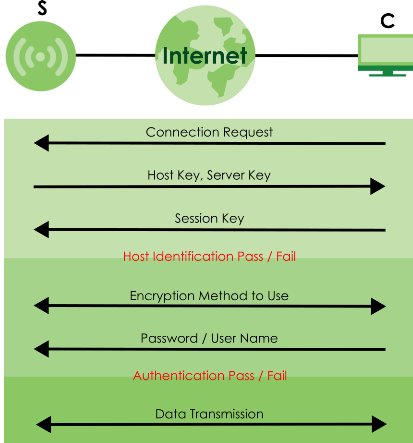
Figure 146 How SSH v1 Works Example
