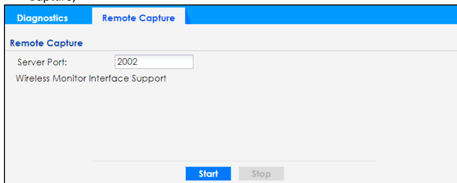
Figure 186 Maintenance > Diagnostics > Remote Capture (Zyxel Device that supports Wireless Remote Capture)
