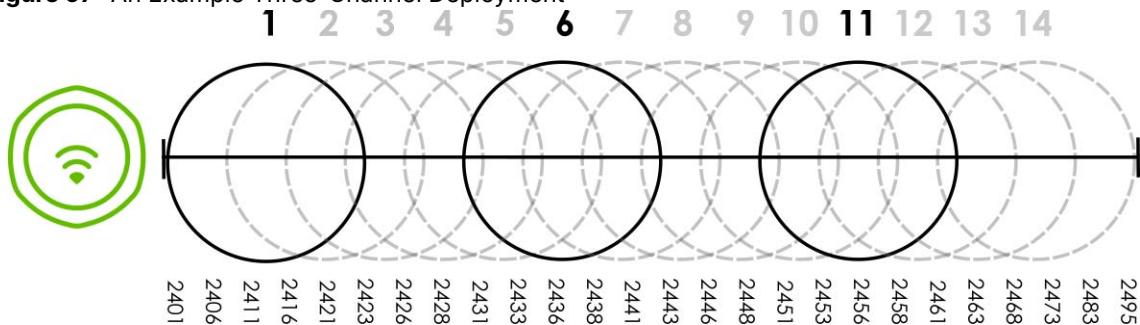
Figure 97 An Example Three-Channel Deployment
