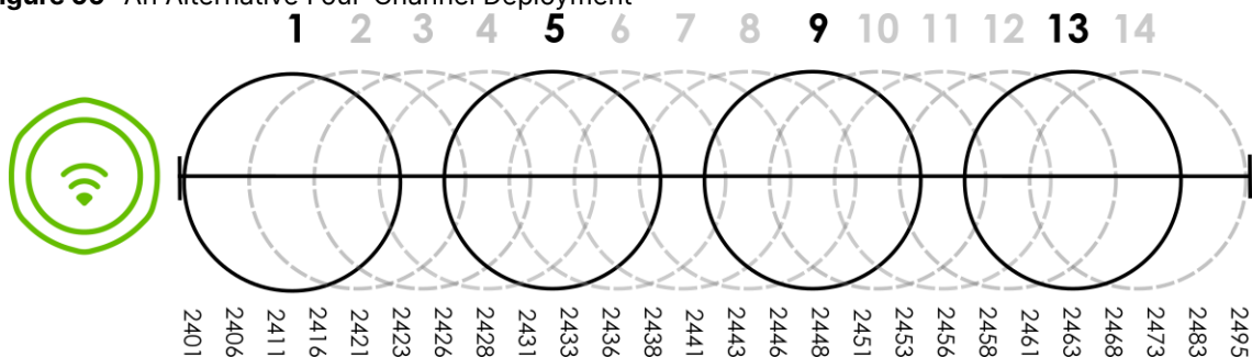
Figure 99 An Alternative Four-Channel Deployment
