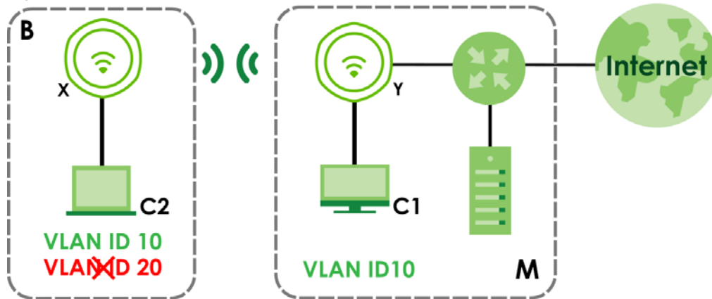
Figure 84 Wireless Bridge VLAN ID Example
