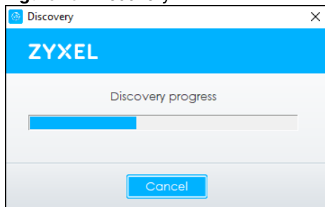
Figure 19 Discovery
