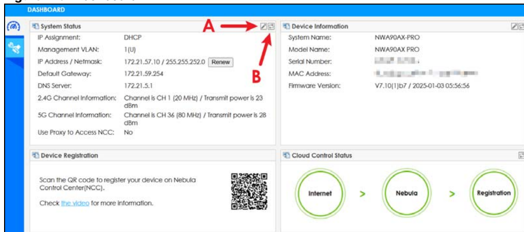
Figure 175 Dashboard
