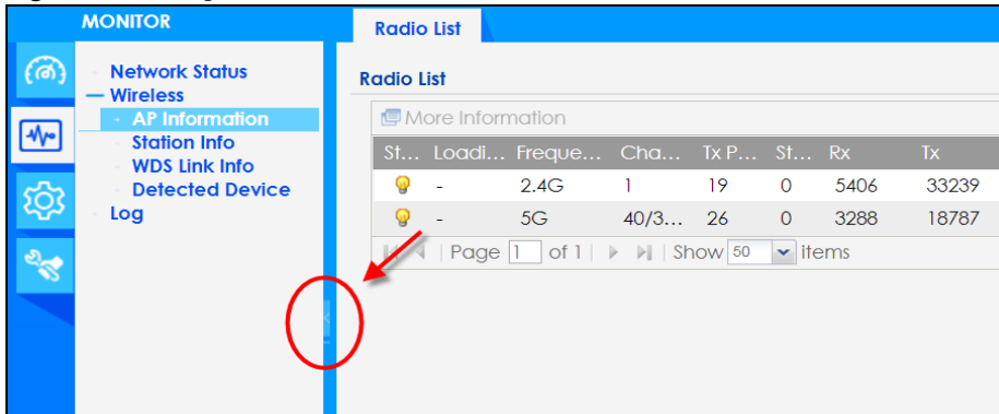
Figure 45 Navigation Panel
