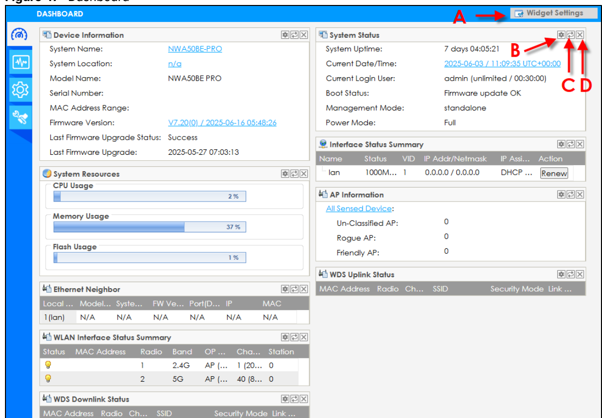
Figure 47 Dashboard
