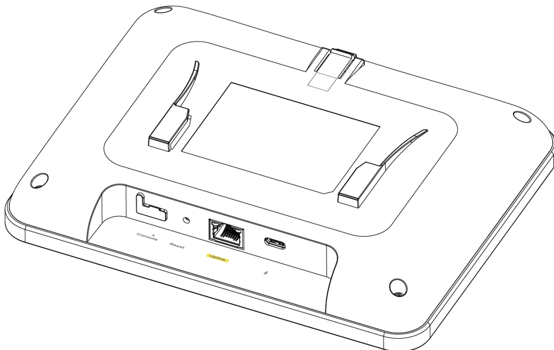
Figure 35 NWA50BE MAX/NWA90BE MAX
