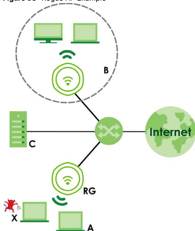
Figure 93 Rogue AP Example
