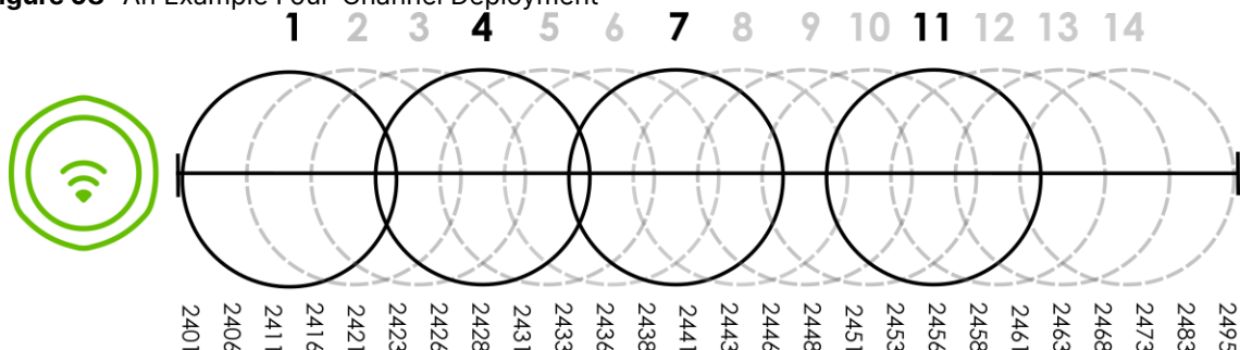
Figure 98 An Example Four-Channel Deployment
