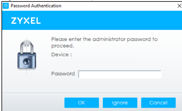
Figure 21 Password Prompt
