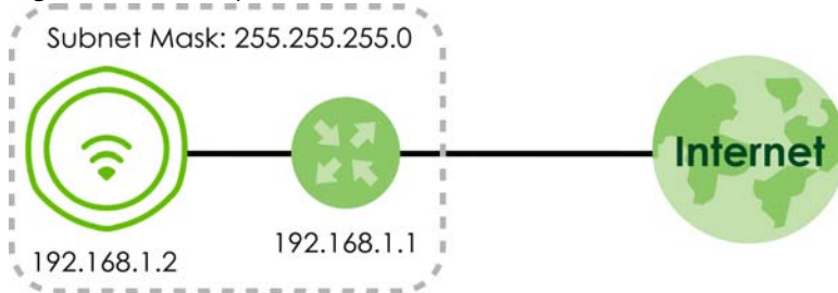
Figure 80 IP Setup
