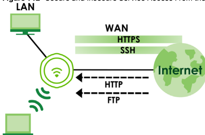
Figure 142 Secure and Insecure Service Access From the WAN
