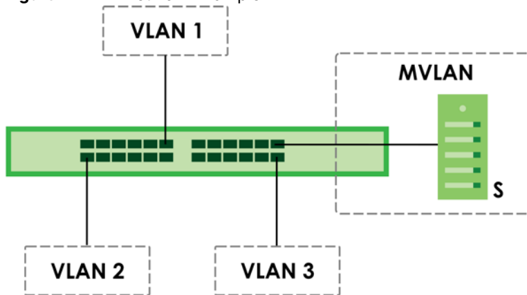
Figure 7 MVR Network Example
