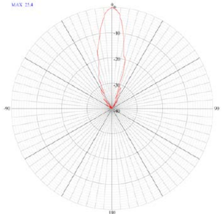
Co-Pol - 0 deg Cut
