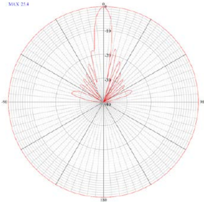
Co-Pol - 90 deg Cut
