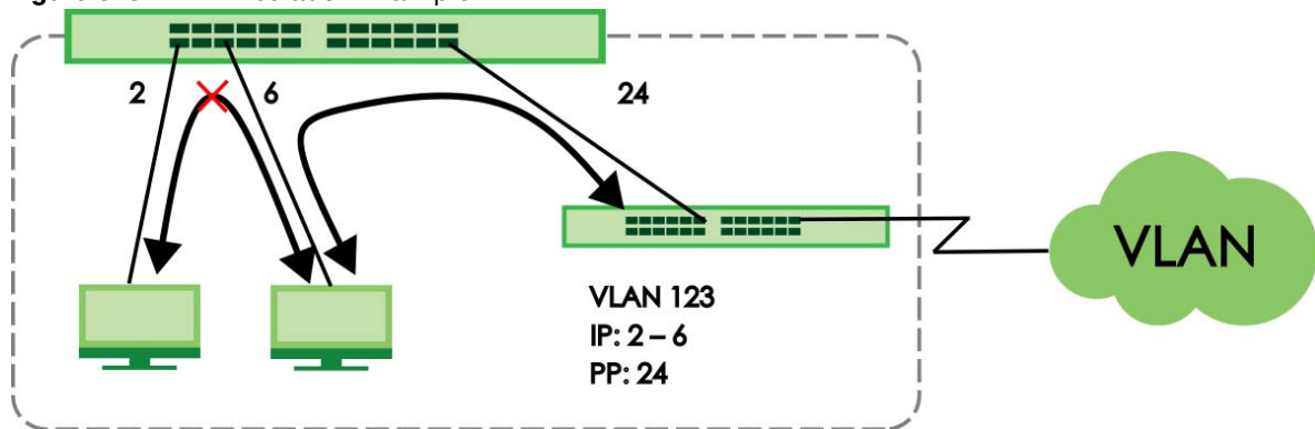
Figure 348 VLAN Isolation Example
