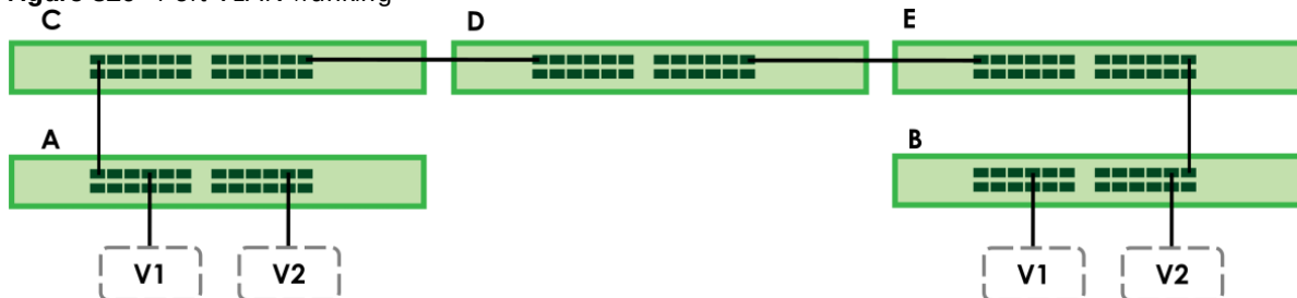
Figure 320 Port VLAN Trunking
