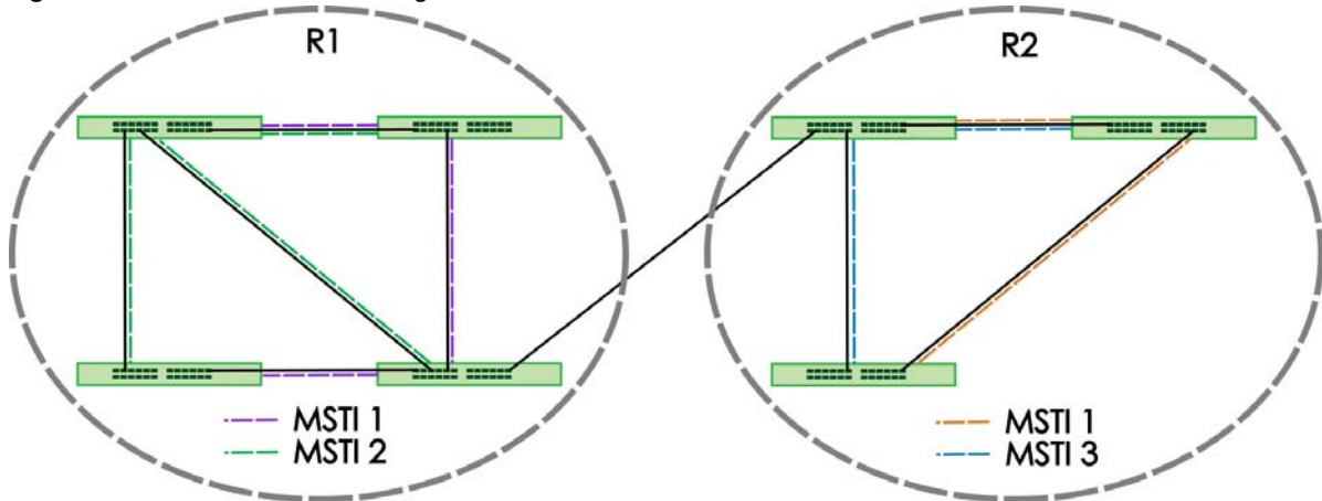
Figure 313 MSTIs in Different Regions
