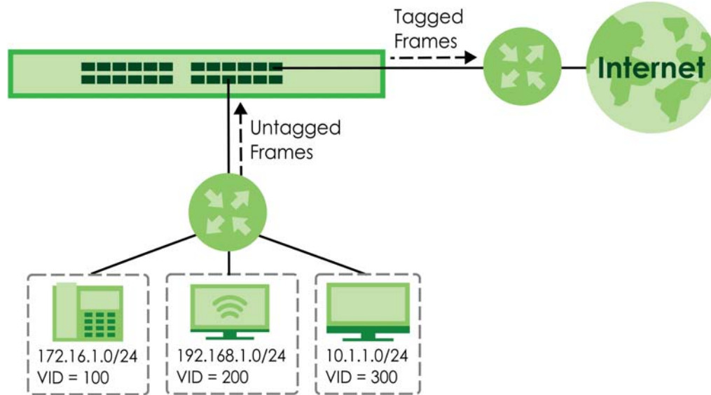
Figure 332 Subnet Based VLAN Application Example
