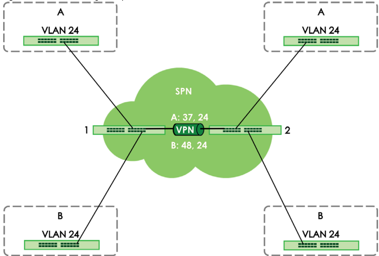
Figure 357 VLAN Stacking Example
