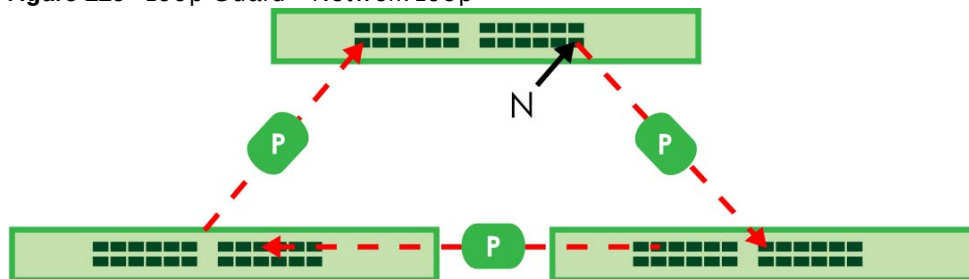
Figure 229 Loop Guard – Network Loop
