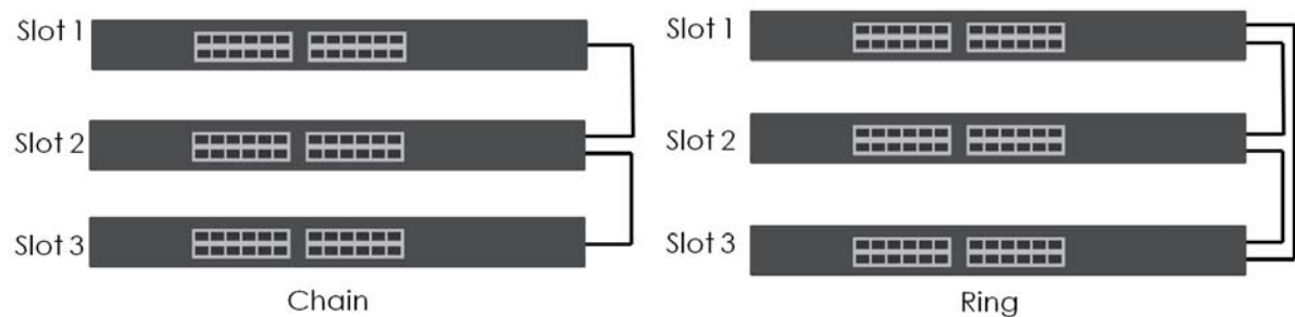
Figure 147 Stacking Topology
