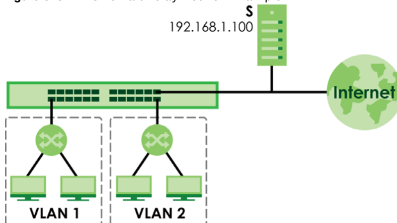
Figure 375 DHCP Smart Relay Network Example
