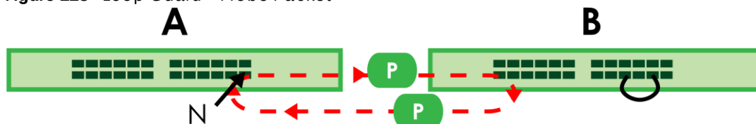
Figure 228 Loop Guard – Probe Packet
