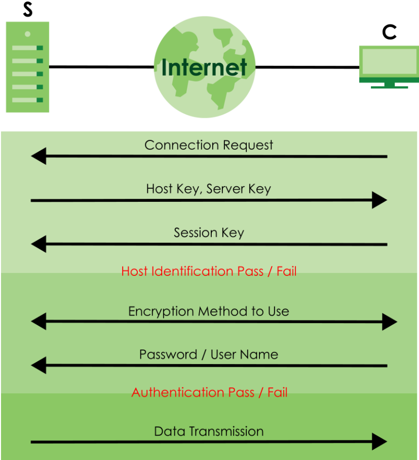
Figure 403 How SSH Works
