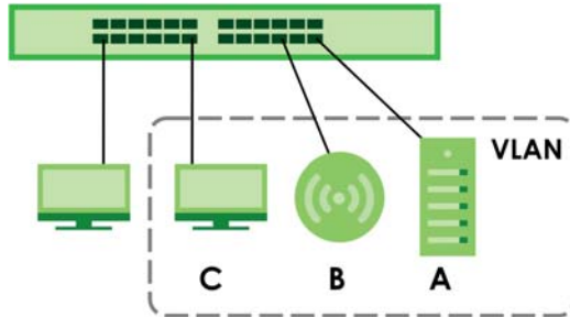
Figure 73 Tutorial: DHCP Snooping Tutorial Overview
