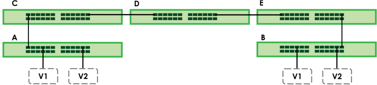
Figure 554 Port VLAN Trunking
