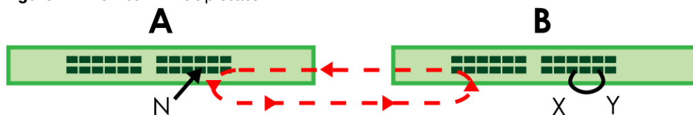
Figure 227 Switch in Loop State
