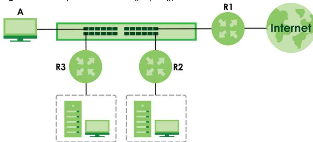
Figure 388 Example of Static Routing Topology
