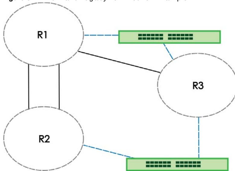
Figure 314 MSTP and Legacy RSTP Network Example
