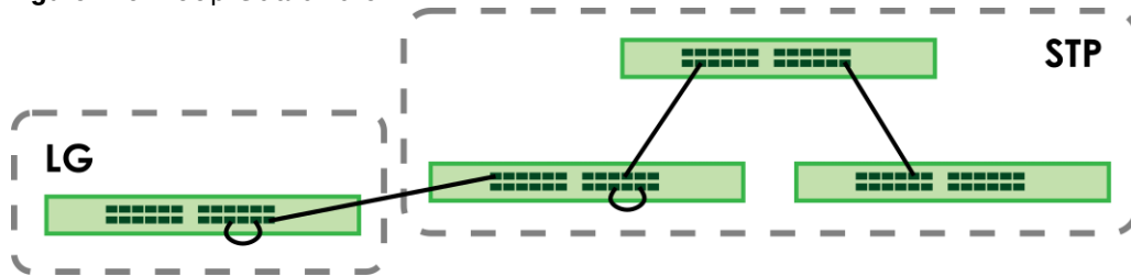
Figure 226 Loop Guard vs. STP
