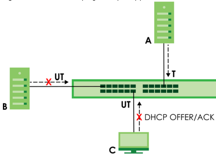
Figure 441 DHCP Snooping Example Application
