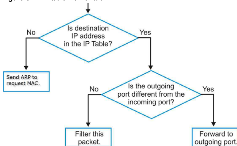
Figure 82 IP Table Flowchart
