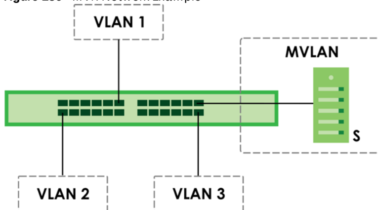
Figure 236 MVR Network Example
