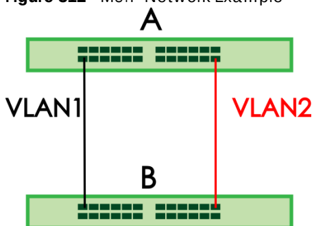
Figure 312 MSTP Network Example
