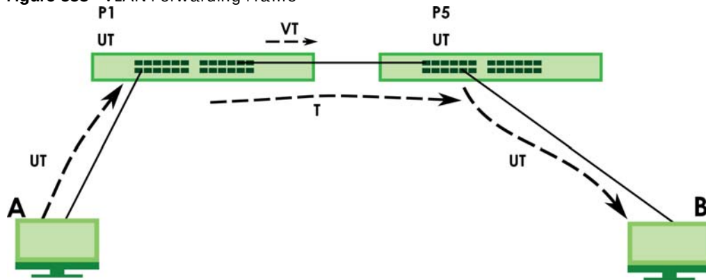
Figure 553 VLAN Forwarding Frame
