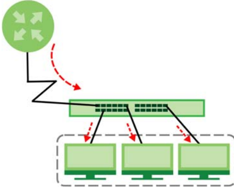
Figure 266 No Multicast Forwarding
