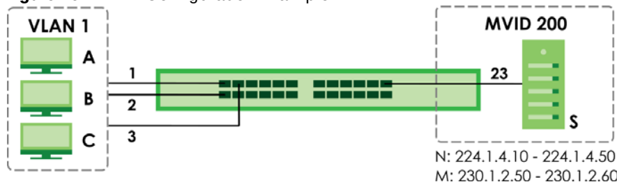
Figure 262 MVR Configuration Example
