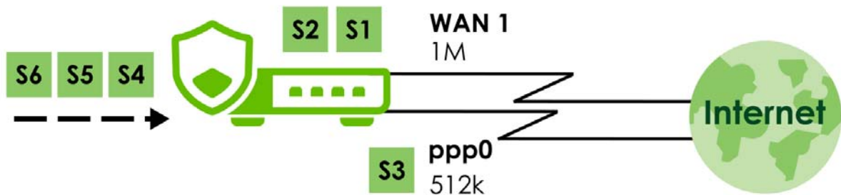
Figure 74 Weighted Round Robin Algorithm Example
