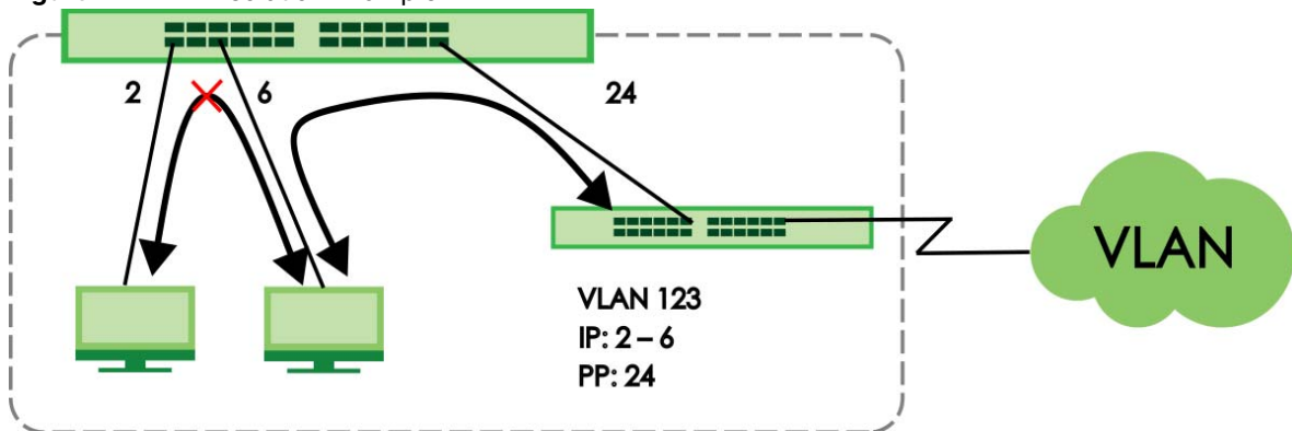
Figure 14 VLAN Isolation Example
