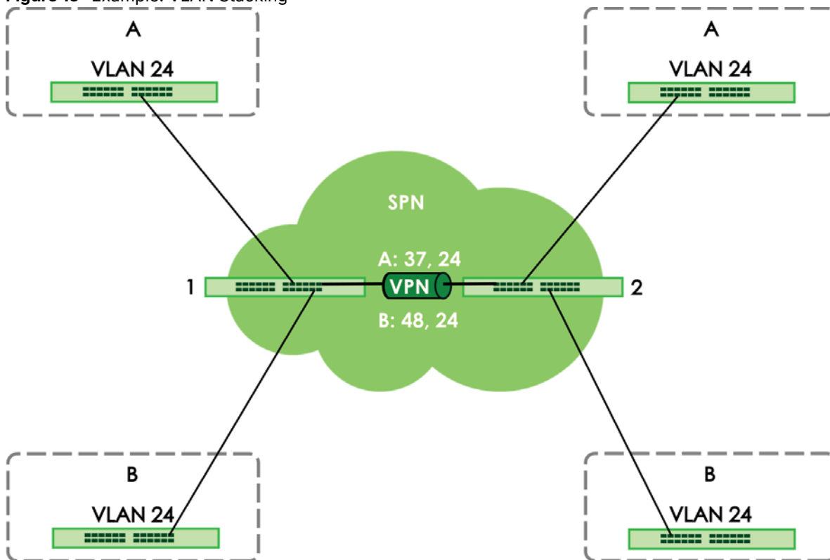
Figure 15 Example: VLAN Stacking
