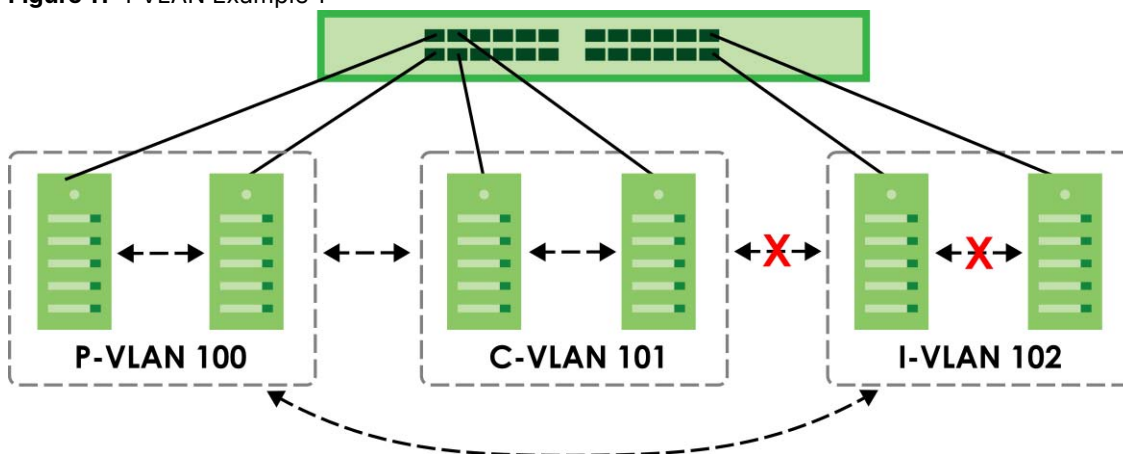
Figure 11 PVLAN Example 1
