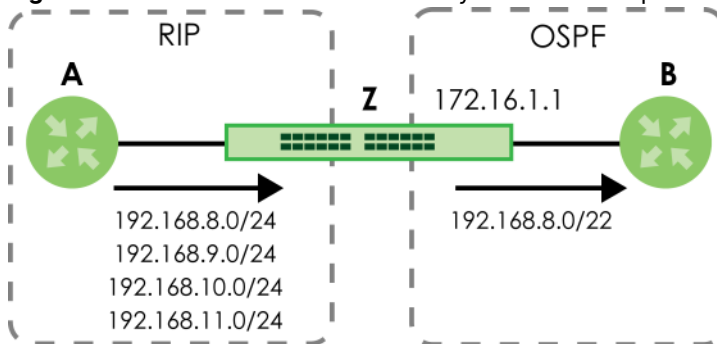
Figure 10 OSPF Redistribution Summary Address Example
