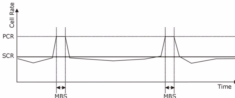
Figure 27 Example of ATM OoS
