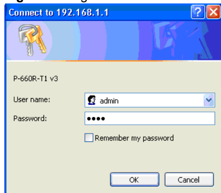
Figure 3 Login Screen
