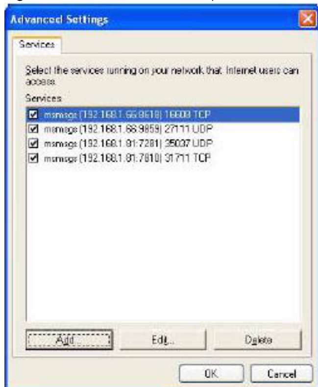
Figure 60 Internet Connection Properties: Advanced Settings
