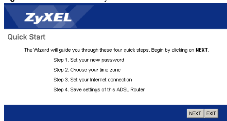
Figure 11 Wizard Summary
