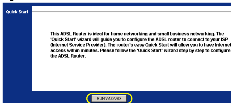
Figure 10 Run Wizard
