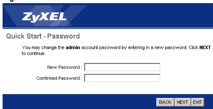
Figure 12 Password
