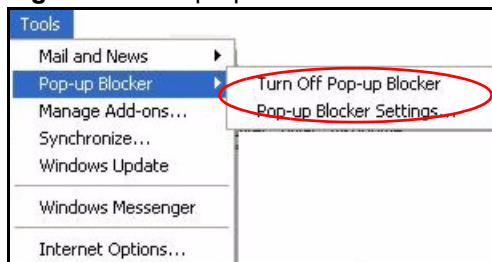
Figure 110 Pop-up Blocker
