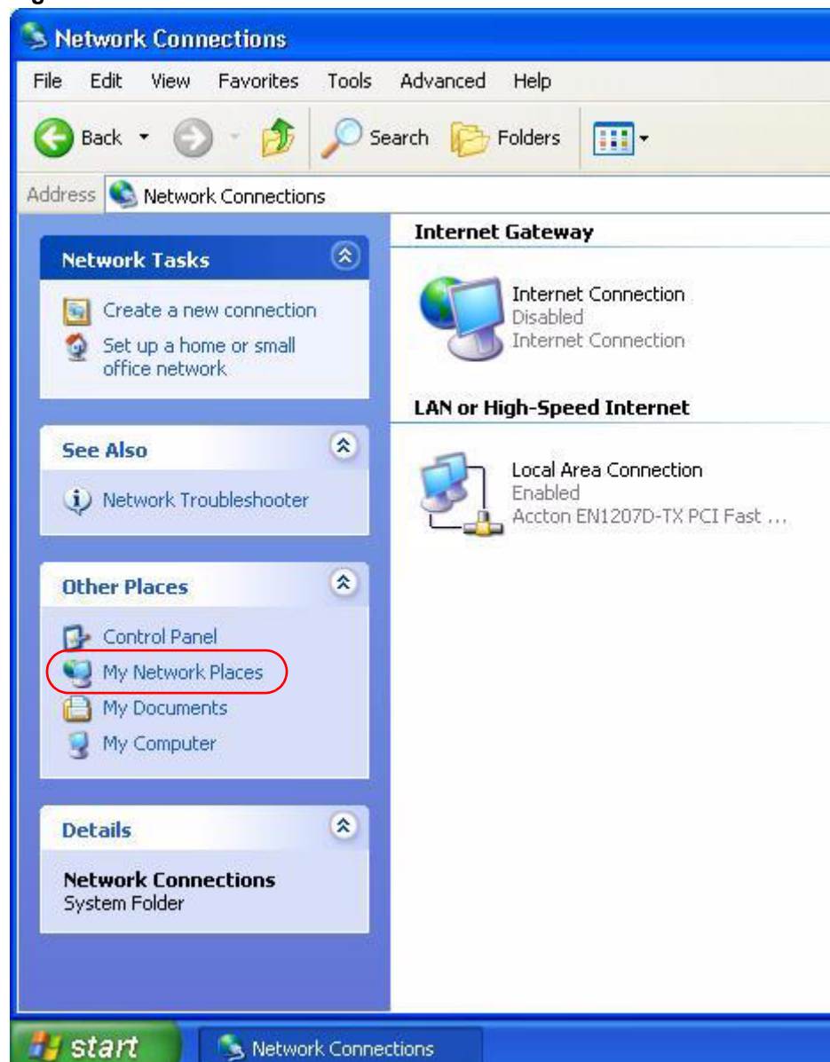
Figure 64 Network Connections
