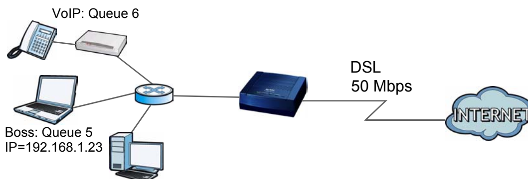
Figure 40 QoS Example
