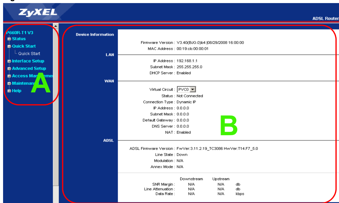
Figure 4 Main Screen
