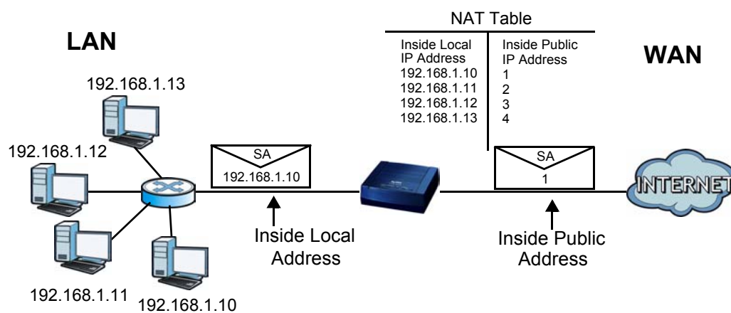
Figure 39 How NAT Works
