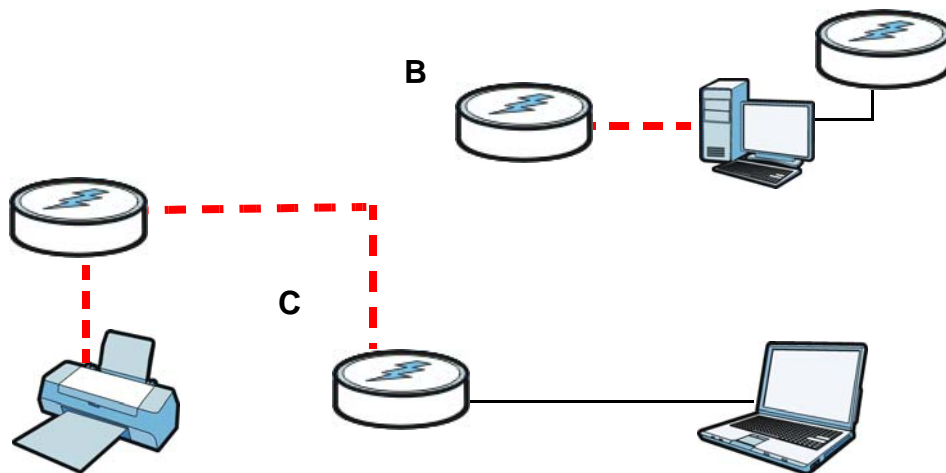
Figure 10 Two Separate Powerline Networks
